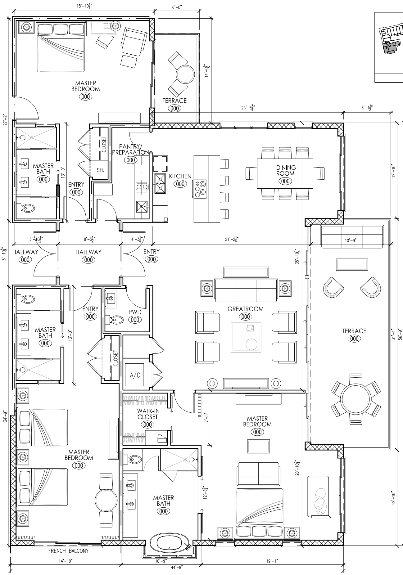
1 ROYAL RESIDENCE FLOOR PLAN SCALE 1/8" = 1'-0" SCALE 0 1' 2' 3' 4' 5' 10' 15'
